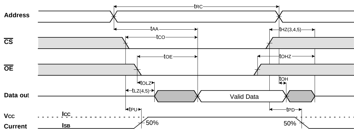
TIMING WAVEFORM OF READ CYCLE(2) ( \overline{\text{WE}}=V_{\text{IH}} )
