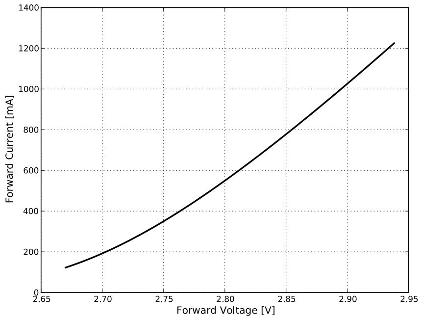
Figure 4c. Typical forward current vs. forward voltage for LUXEON CZ Mint at T_j=85^\circ\text{C} .
