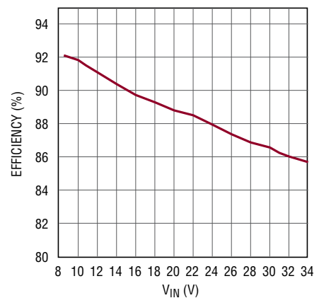
Efficiency vs V_{IN} , Buck Mode, 6.8V at 1A LED String
