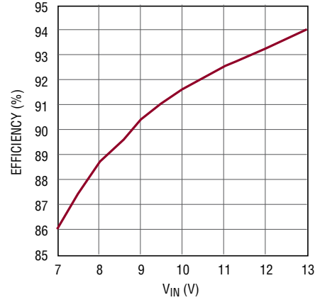
Efficiency vs V_{IN} , Boost Operation, 13.4V at 1A LED String
