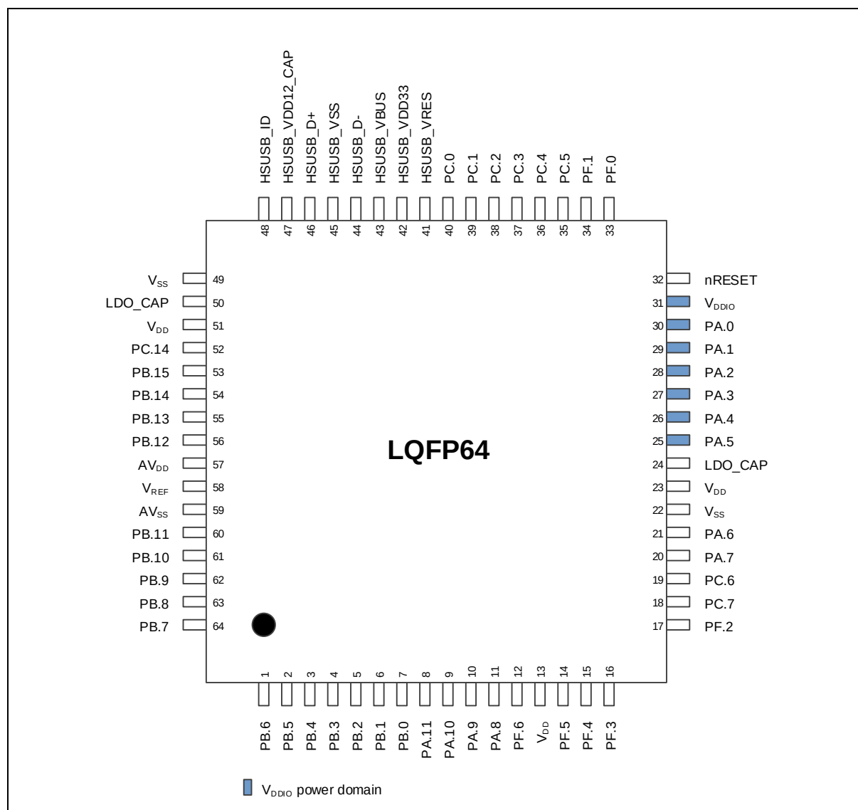
Figure 4.1-8 NuMicro® M483 CAN Series LQFP 64-pin Diagram
