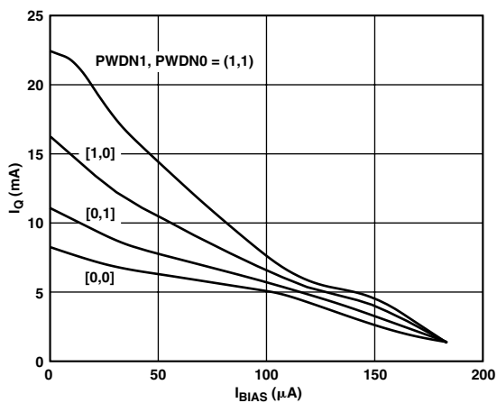
Figure 34. I_Q vs. I_{BIAS} Current; V_S = \pm 12V
