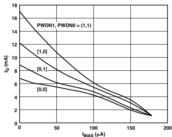
Figure 35. I_Q vs. I_{BIAS} Current; V_S = \pm 6V
