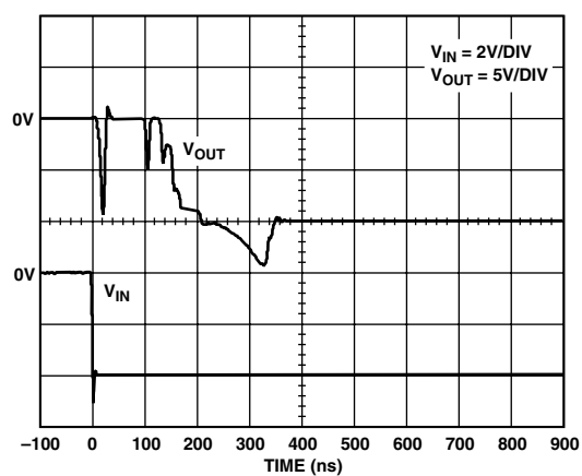
Figure 33b. Overload Recovery; V_S = \pm 12V , G = +5 , R_L = 100\Omega
