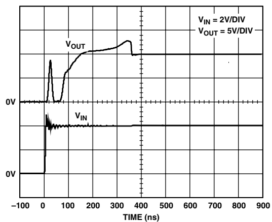
Figure 33a. Overload Recovery; V_S = \pm 12V , G = +5 , R_L = 100\Omega
