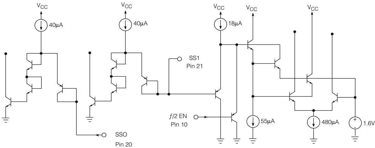
Fig. 8 Pins 20, 21 and 10
