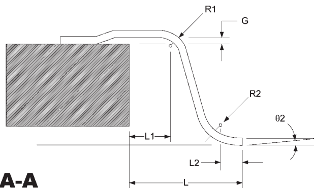
Gullwing Lead
