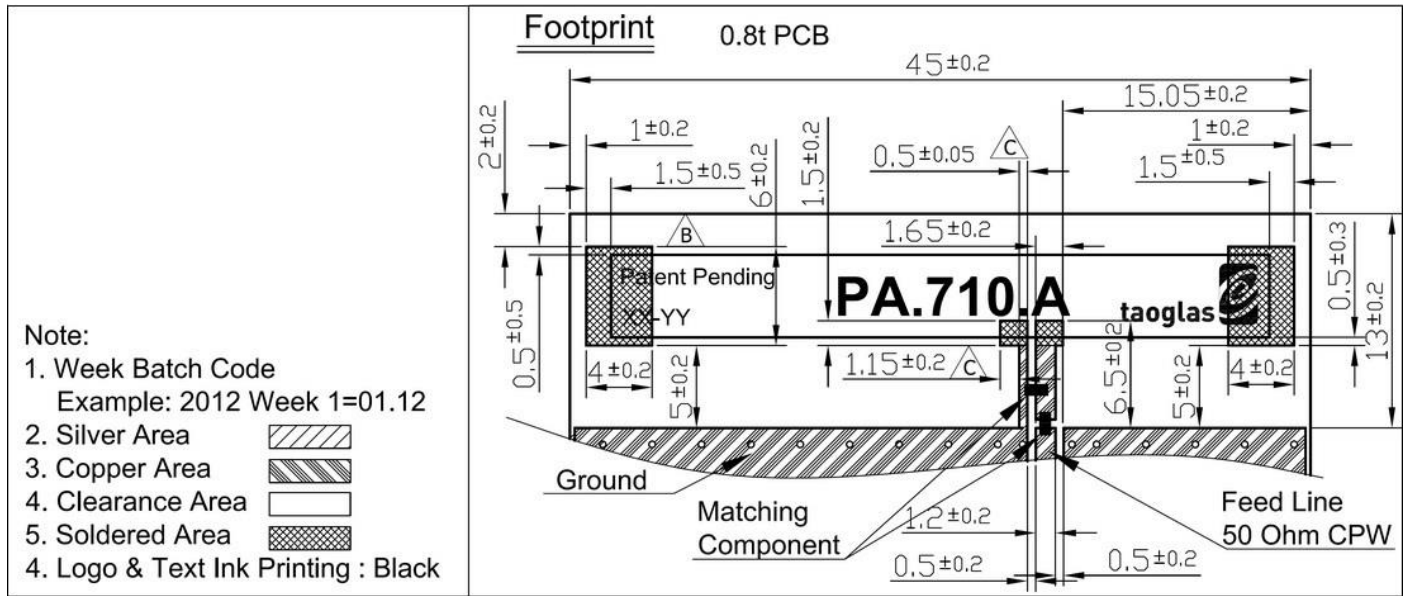
Figure 15. Layout dimensions of the Warrior PA.710.A Antenna.
