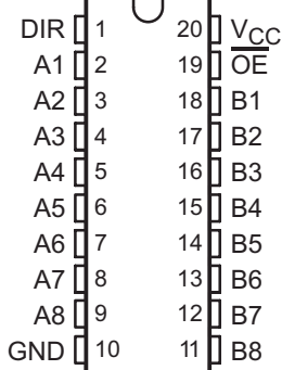
SN54AHCT245 . . . J OR W PACKAGE SN74AHCT245 . . . DB, DGV, DW, N, NS, OR PW PACKAGE (TOP VIEW)
