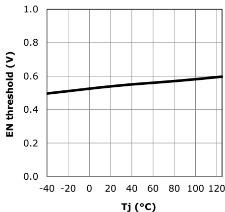
Fig. 8: Enable threshold versus temperature
