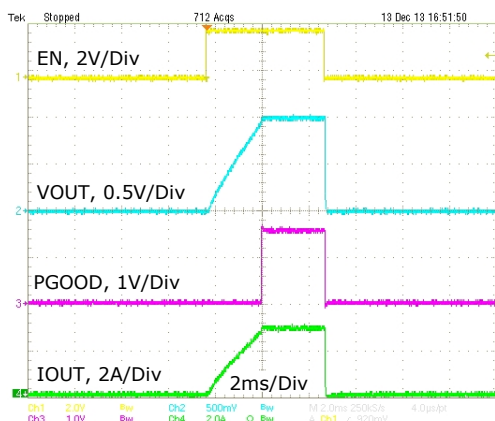
Fig. 11: Enable turn on/off, 3A, 1.5VIN, 1VOUT
