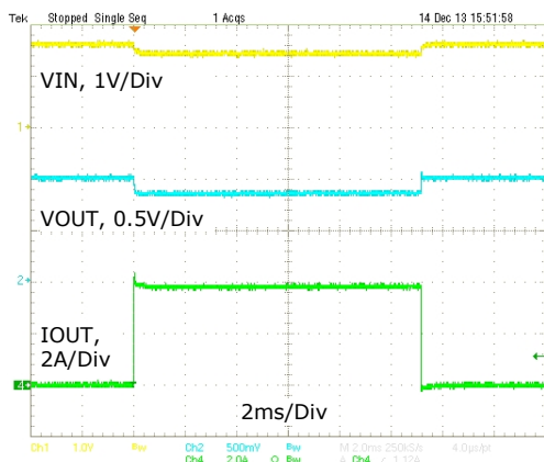
Fig. 13: Current limit, 1.5VIN, 1VOUT
