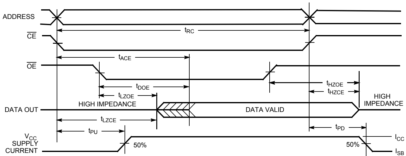
Figure 5. Read Cycle No. 2: \overline{\text{OE}} Controlled [19, 20]
