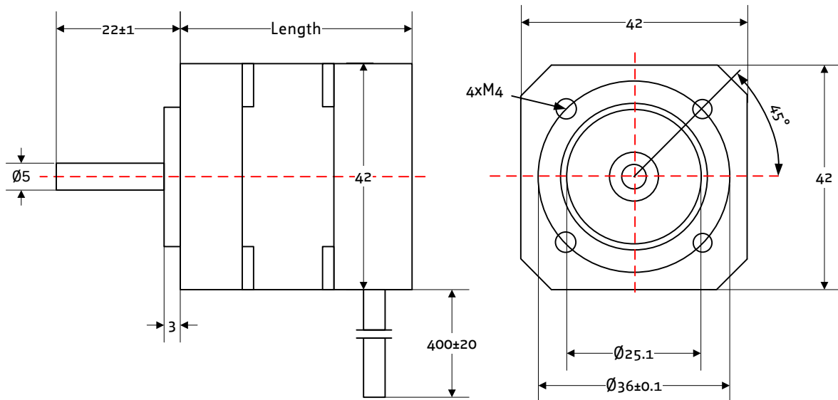
Figure 4.1: Dimensions (all values in mm)
