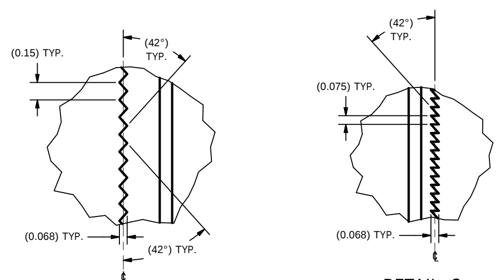
DETAIL F APERTURE LEFT EDGE SCALE 60 : 1
