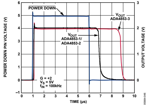
Figure 47. Enable/Disable Time
