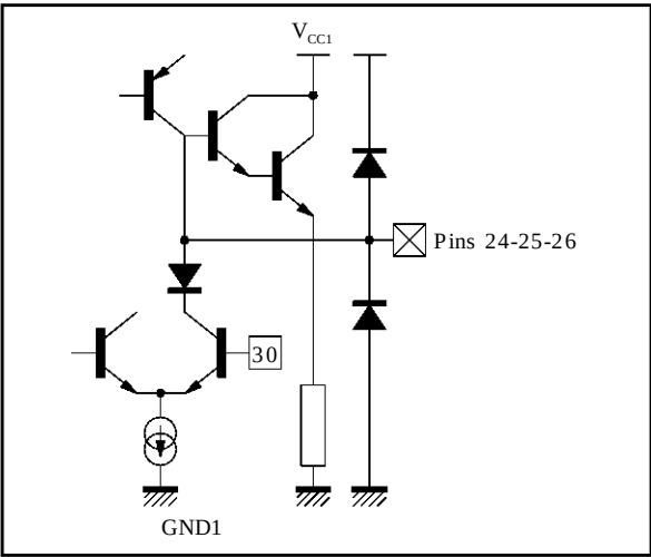
Figure 23 : Pin 30 - ICAT
