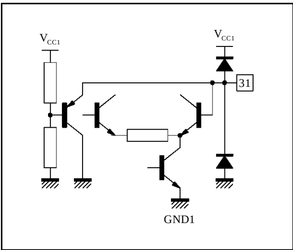
Figure 24 : Pin 31 - BCL
