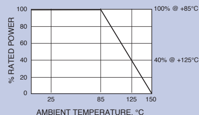
Derating Curve:
