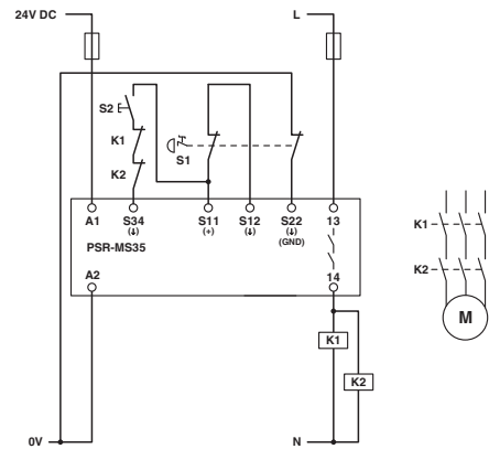
Application drawing
