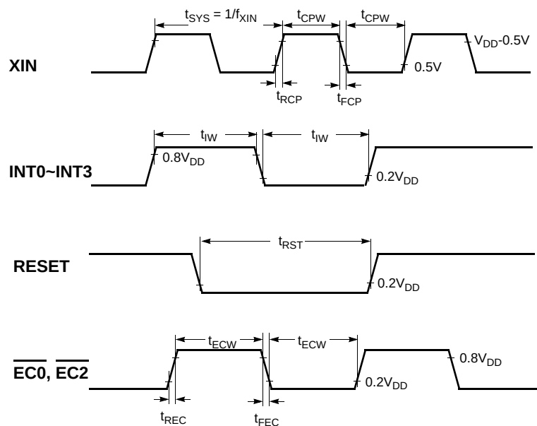
Figure 7-1 Timing Chart
