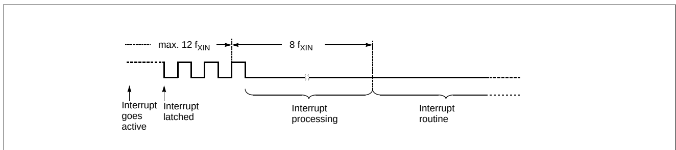
Figure 16-8 Interrupt Response Timing Diagram
