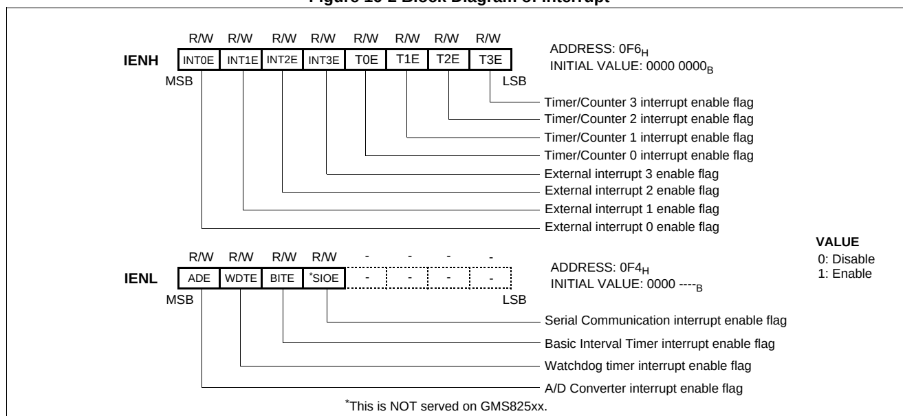
Figure 16-3 Interrupt Enable Flag
