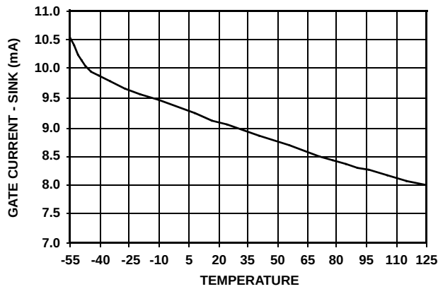
FIGURE 16. I_{GATE} (SINK) vs TEMPERATURE
