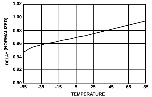
FIGURE 19. t_{DELAYi} vs TEMPERATURE
