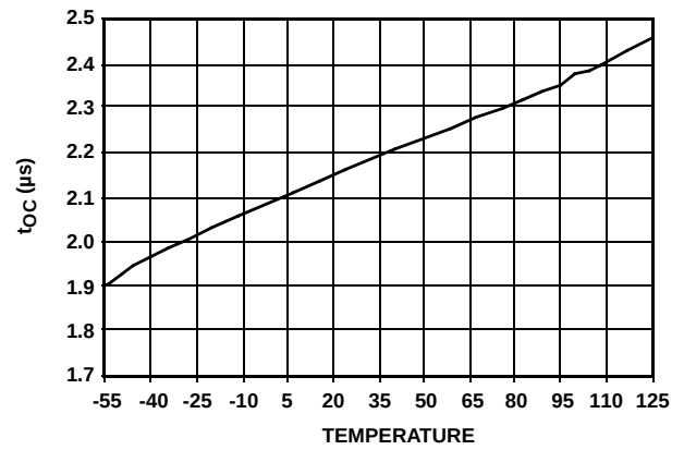
FIGURE 17. t_{FOC} vs TEMPERATURE
