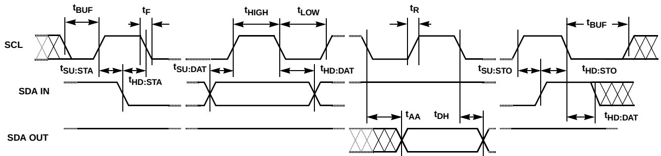
FIGURE 7. BUS TIMING
