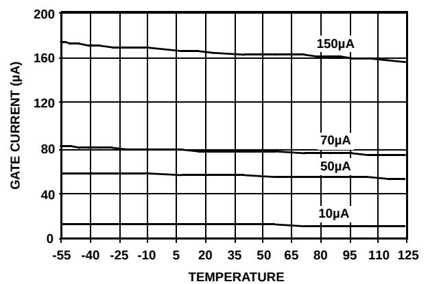
FIGURE 15. I_{\text{GATE}} (SOURCE) vs TEMPERATURE
