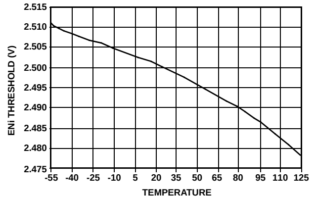
FIGURE 13. \overline{\text{ENI}} THRESHOLD vs TEMPERATURE
