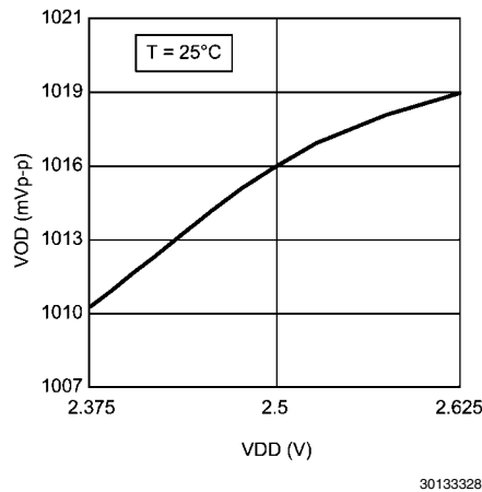
FIGURE 8. Output Differential Voltage (VOD = 1.0 Vp-p) vs. Supply Voltage (VDD)
