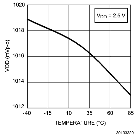
FIGURE 9. Output Differential Voltage (VOD = 1.0 Vp-p) vs. Temperature
