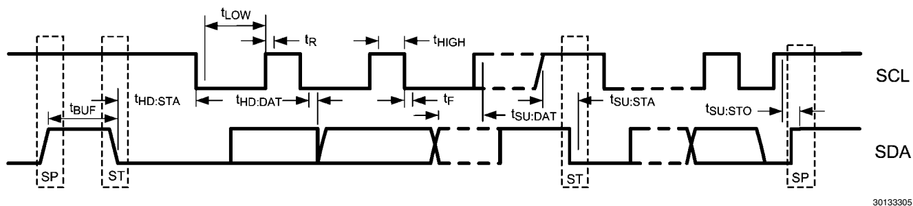
FIGURE 4. SMBus Timing Parameters
