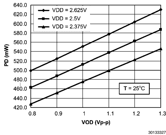
FIGURE 7. Power Dissipation (PD) vs. Output Differential Voltage (VOD)
