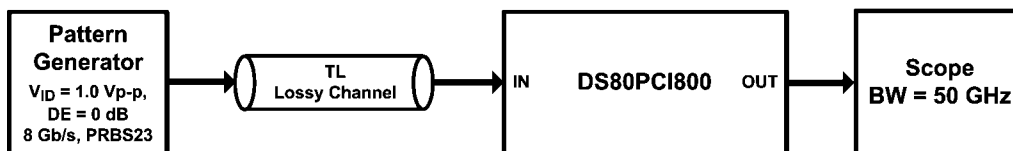
FIGURE 10. Test Setup Connections Diagram
