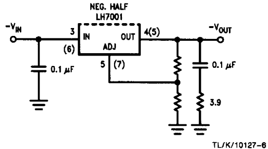
FIGURE 2. Choice of Capacitors for Stable Operation
