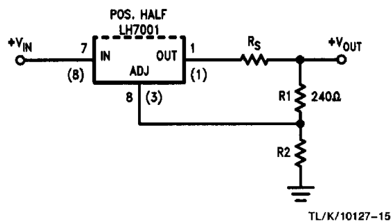
FIGURE 8. Positive Regulator with Line Resistance in Output Lead*
