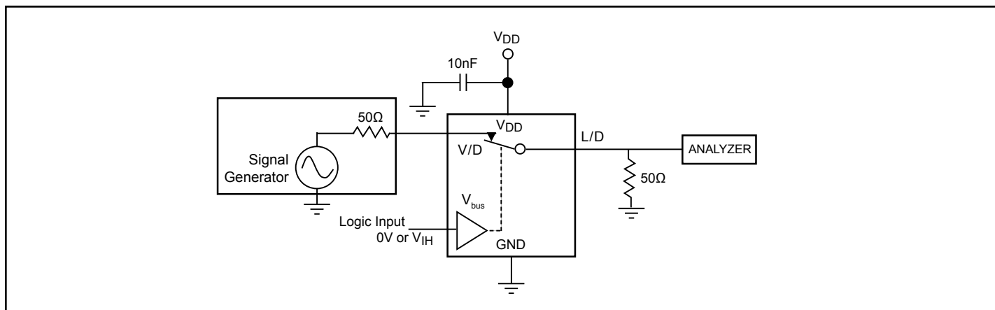
Figure 9. Bandwidth
