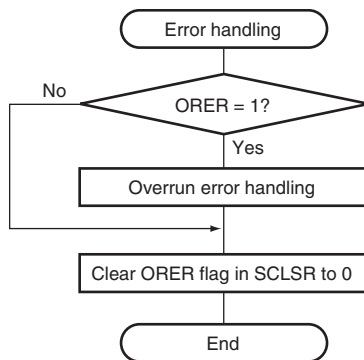
Figure 16.16 Sample Flowchart for Receiving Serial Data (2)
