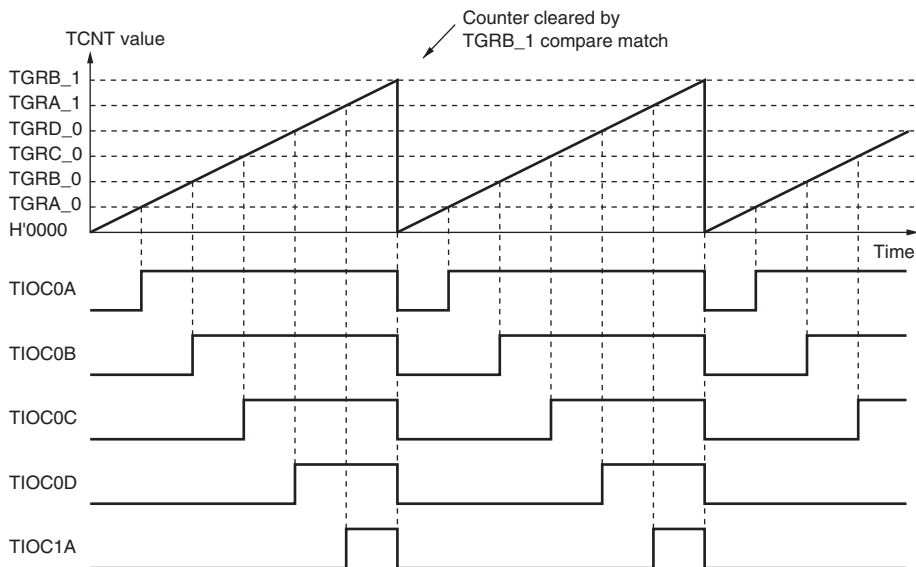
Figure 11.27 Example of PWM Mode Operation (2)
