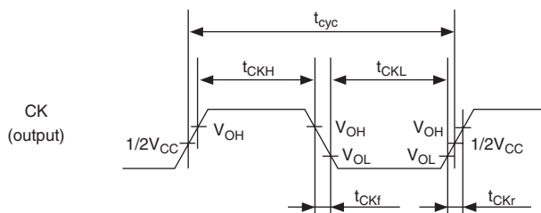
Figure 28.2 CK Clock Output Timing
