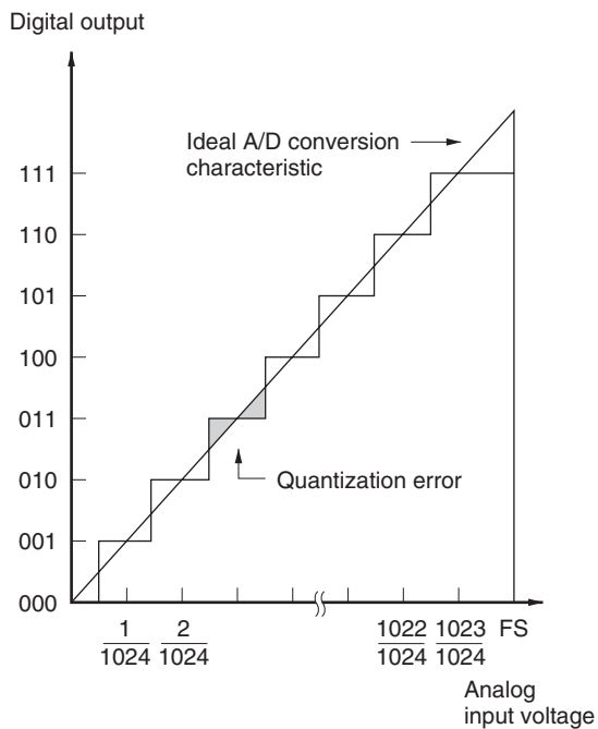
Figure 19.5 Definitions of A/D Conversion Accuracy
