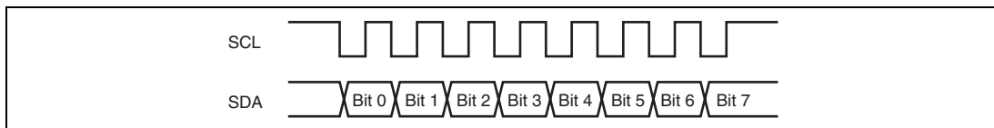
Figure 18.13 Clock Synchronous Serial Transfer Format
