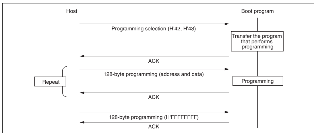
Figure 23.26 Sequence of Programming
