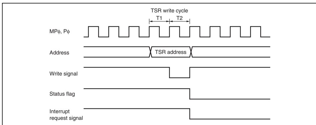
Figure 11.116 Timing for Status Flag Clearing by CPU (Channel 5)
