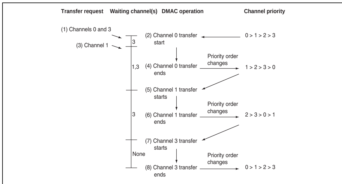
Figure 10.4 Changes in Channel Priority in Round-Robin Mode
