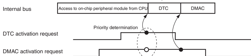
Figure 9.49 Bus Arbitration when DTC and DMAC Compete during External Space Access from CPU
