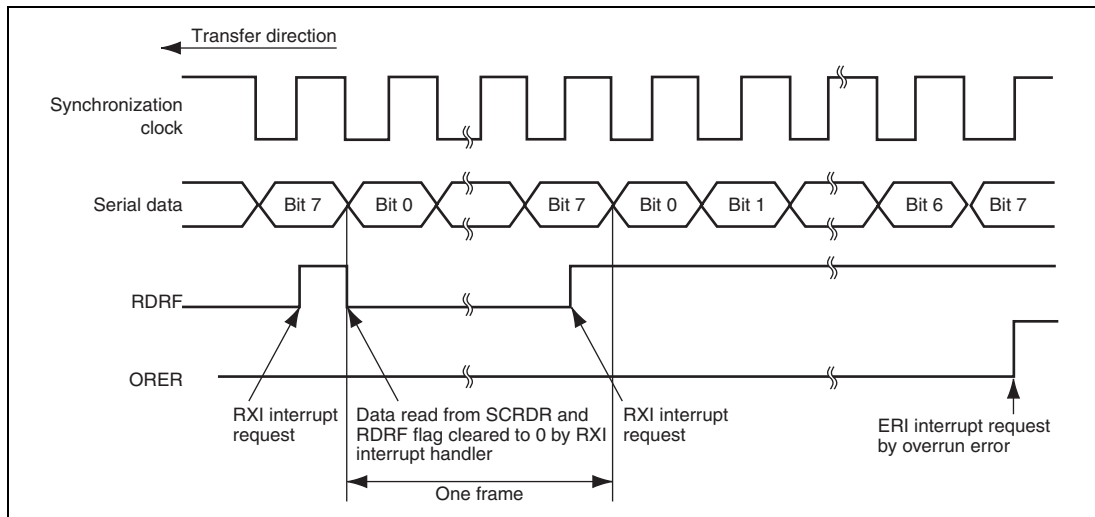
Figure 15.13 Example of SCI Receive Operation
