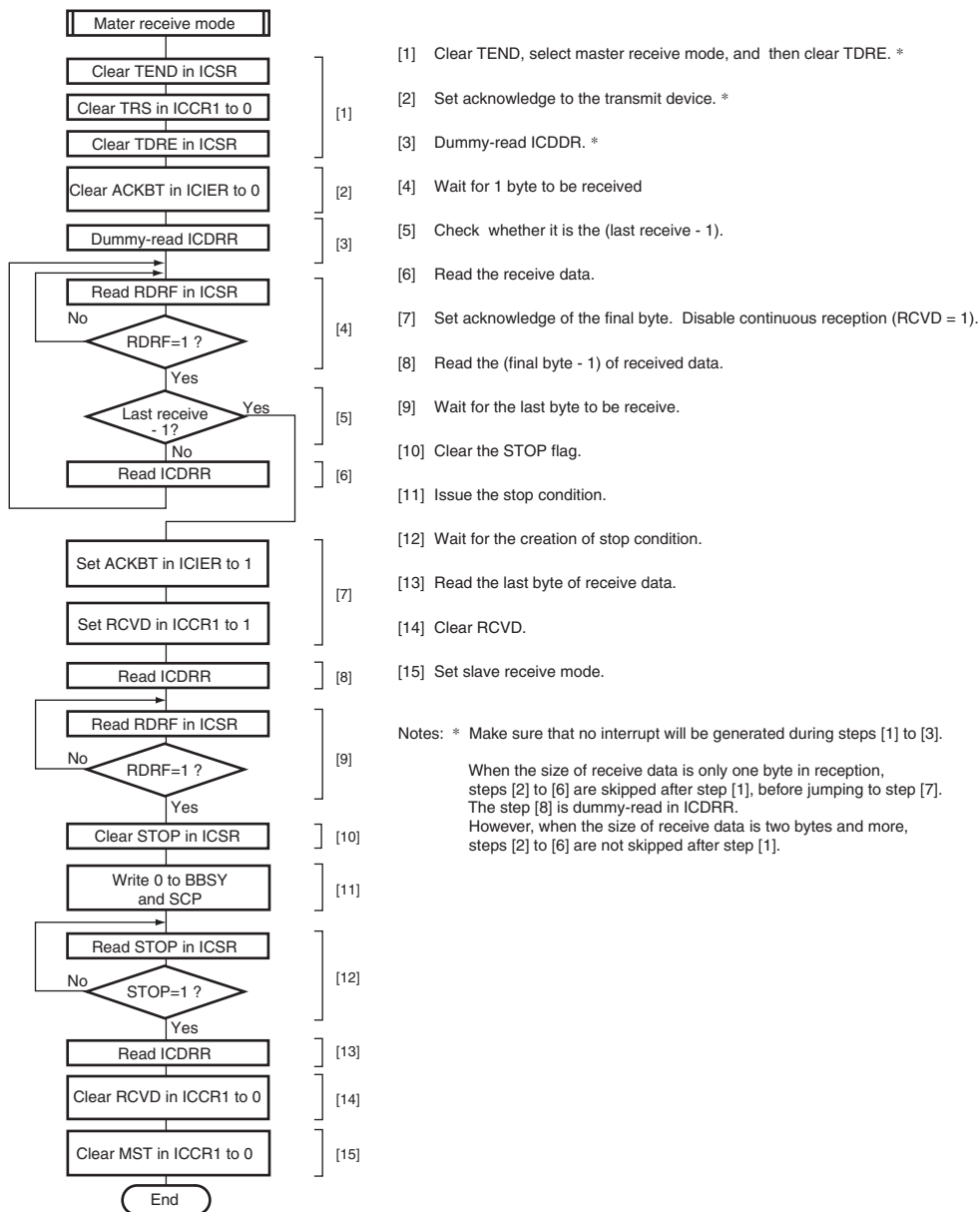
Figure 18.19 Sample Flowchart for Master Receive Mode
