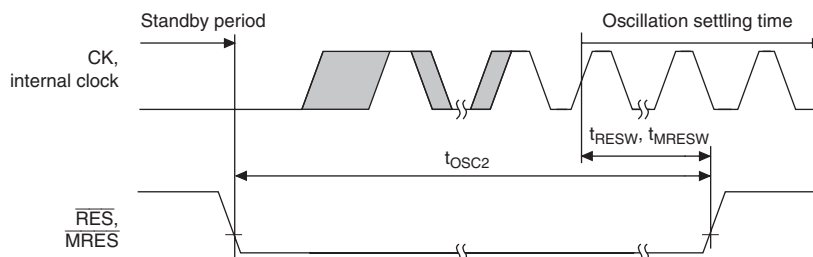
Figure 28.3 Power-On Oscillation Settling Timing
