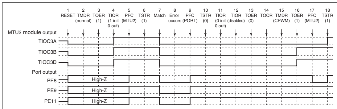
Figure 11.141 Error Occurrence in Normal Mode, Recovery in Complementary PWM Mode
