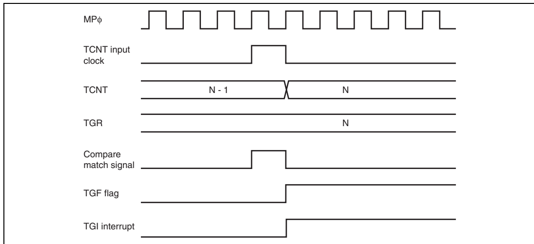
Figure 11.110 TGI Interrupt Timing (Compare Match) (Channel 5)
