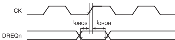
Figure 28.45 DREQ Input Timing
