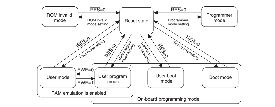
Figure 23.2 Mode Transition of Flash Memory
