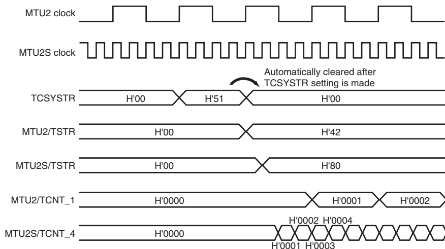
Figure 11.84 (4) Example of Synchronous Counter Start Operation (MTU2-to-MTU2S Clock Frequency Ratio = 1:4)
