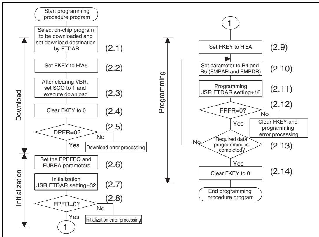
Figure 23.11 Programming Procedure
