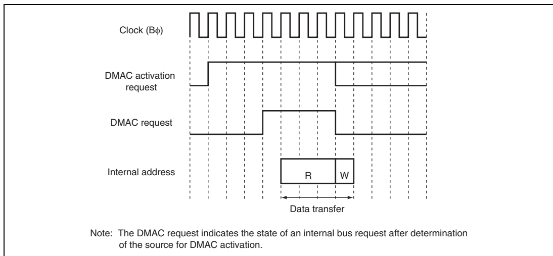
Figure 10.21 Example of DMAC Operation Timing— Activation by an On-Chip Peripheral Module (in the Case of Cycle Stealing Transfer, Dual Address Mode, Low-Level Detection, I\phi:B\phi:P\phi = 1:1/2:1/2, and Data Transfer from On-Chip Peripheral Module to On-Chip RAM)
