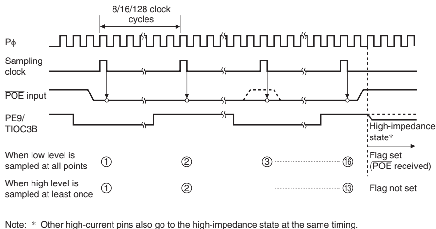
Figure 13.3 Low-Level Detection Operation
