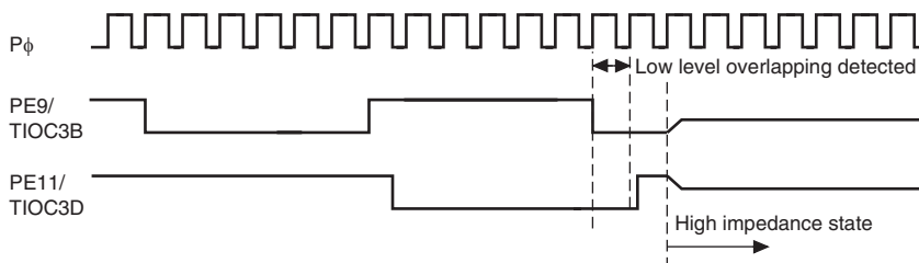
Figure 13.4 Output-Level Compare Operation
