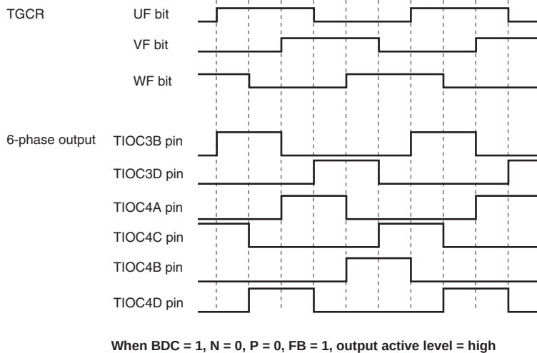
Figure 11.71 Example of Output Phase Switching by Means of UF, VF, WF Bit Settings (1)
