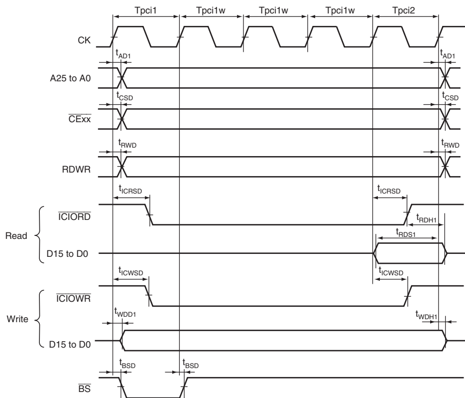
Figure 28.43 PCMCIA I/O Card Interface Bus Timing
