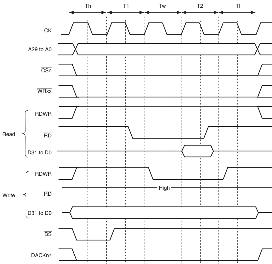
Figure 9.34 Byte Selection SRAM Wait Timing (BAS = 1, SW[1:0] = 01, WR[3:0] = 0001, HW[1:0] = 01)
