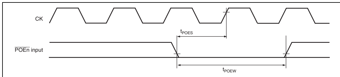
Figure 28.59 \overline{POE} Input Timing
