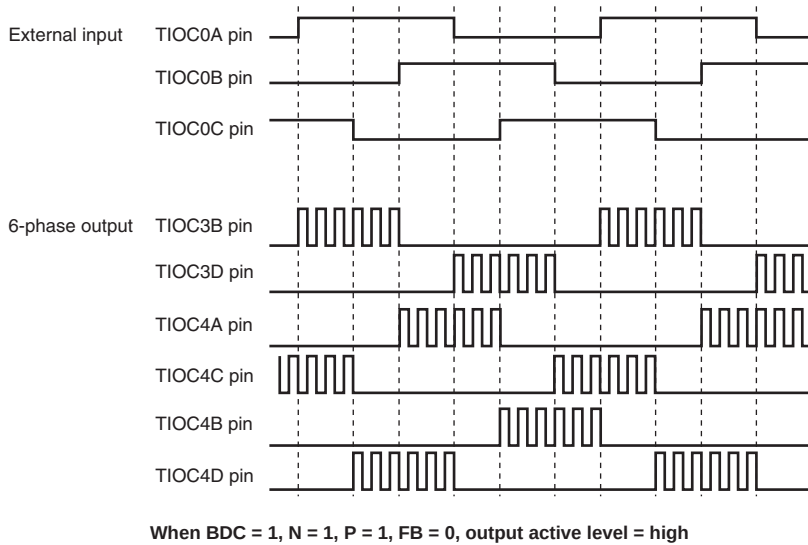
Figure 11.70 Example of Output Phase Switching by External Input (2)
