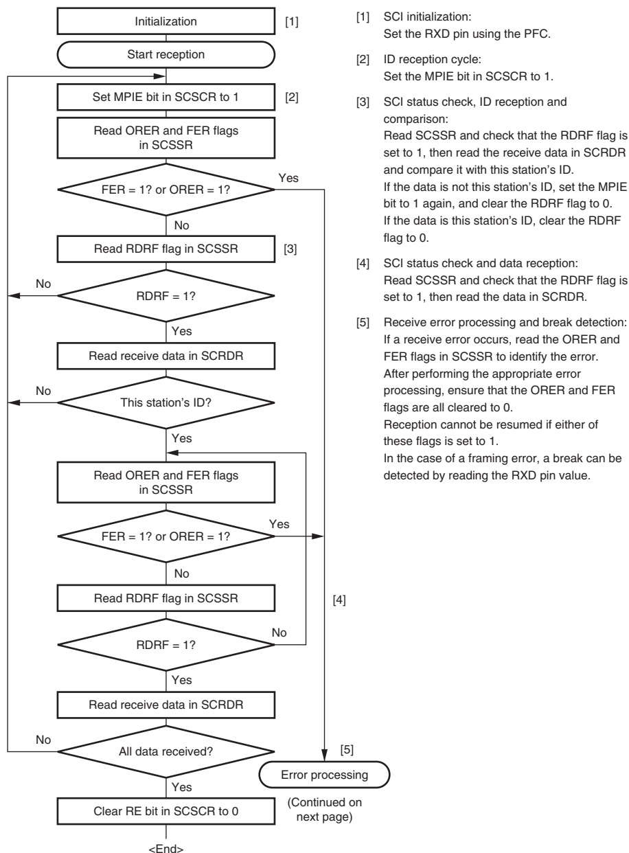
Figure 15.18 Sample Multiprocessor Serial Reception Flowchart (1)
