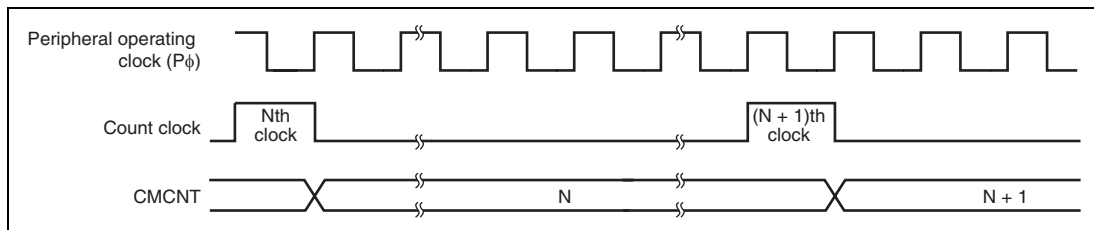
Figure 20.3 Count Timing
