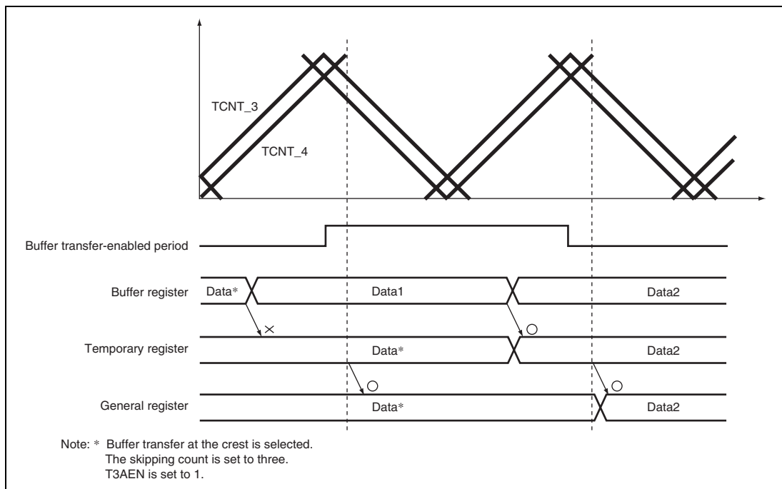
Figure 11.77 Example of Operation when Buffer Transfer is Linked with Interrupt Skipping (BTE1 = 1 and BTE0 = 0)
