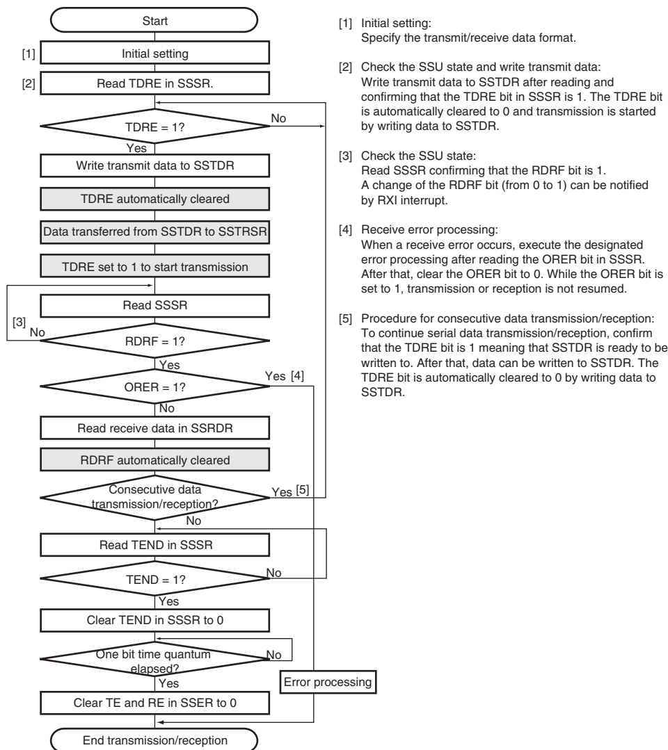
Figure 17.17 Flowchart Example of Simultaneous Transmission/Reception (Clock Synchronous Communication Mode)
