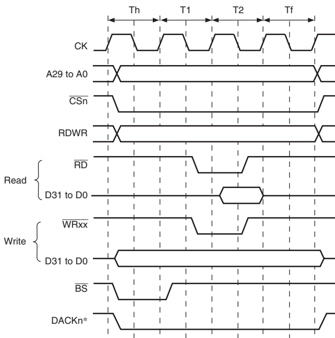
Figure 9.10 \overline{\text{CSn}} Assert Period Extension
