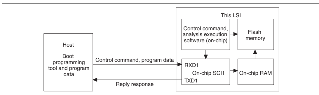
Figure 23.6 System Configuration in Boot Mode
