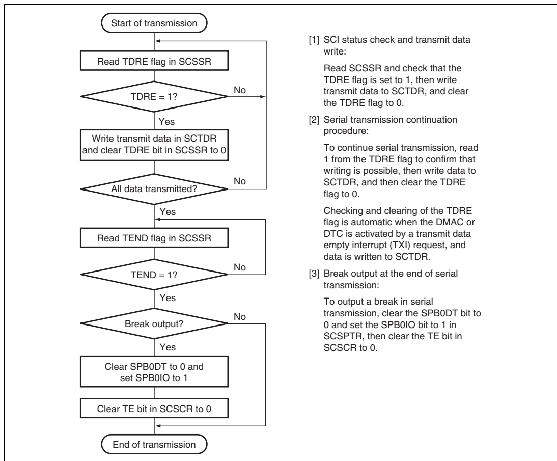
Figure 15.4 Sample Flowchart for Transmitting Serial Data
