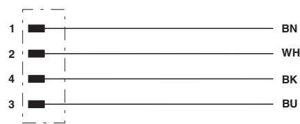
Circuit diagram
