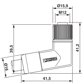
Dimensional drawing
