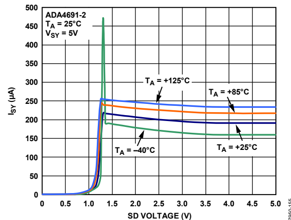
Figure 60. Supply Current vs. Temperature, V_{SY} = 5\text{V}
