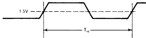
FIGURE 1: VCOCLK TIMING
