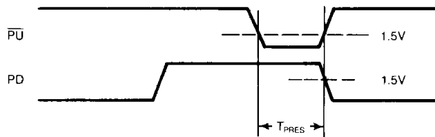
FIGURE 4: PUMPDOWN TO PUMPUP TIMING
