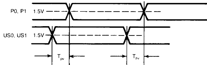
FIGURE 2: PRECOMP VALUE TIMING
