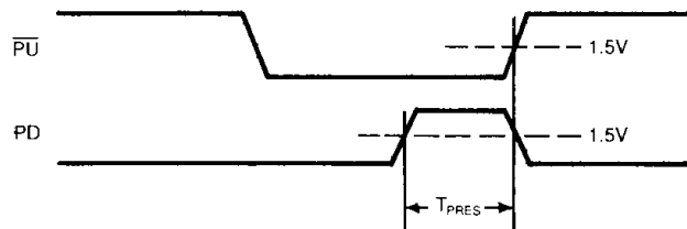
FIGURE 3: PUMPUP TO PUMPDOWN TIMING
