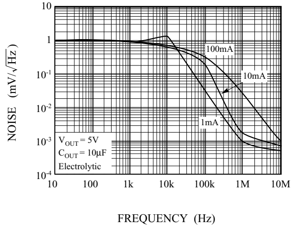
f - NOISE (2)
