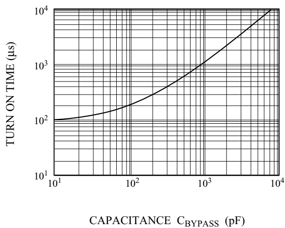
C_{BYPASS} - TIME
