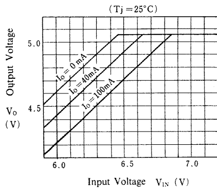
78L05 Dropout Characteristics
