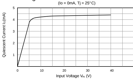
78L05 Quiescent Current vs. Input Voltage
