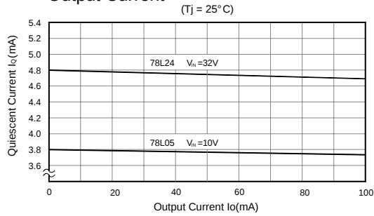
78L05 / L24 Quiescent Current vs. Output Current
