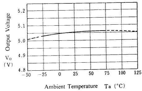
78L05 Output Voltage vs. Temperature
