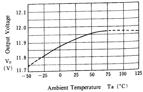
78L12 Output Voltage vs. Temperature
