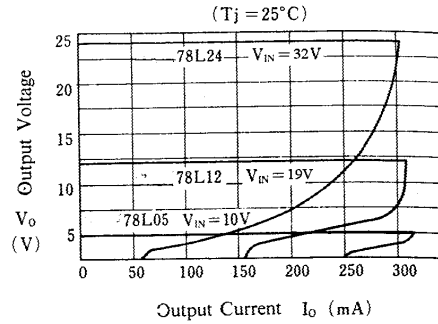
78L05/L12/L24 Load Characteristics
