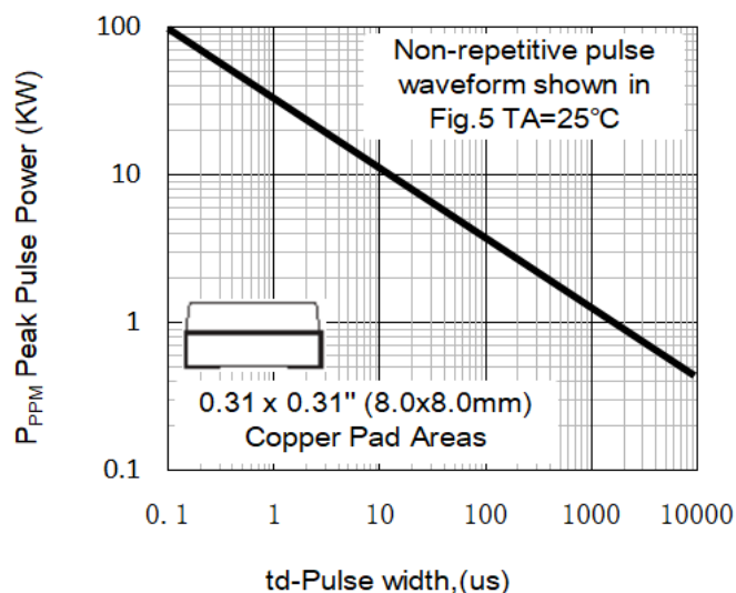
Fig. 4 Peak Pulse Power Rating
