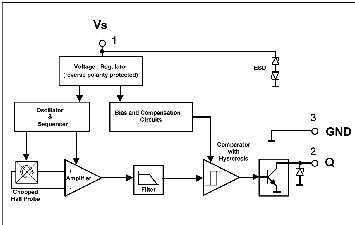
Figure 1: Block Diagram
