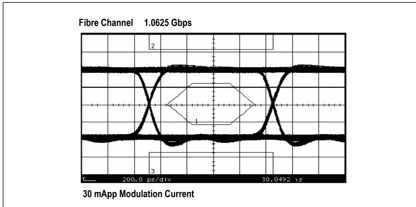
Figure 3-3. Fibre Channel 1.0625 Gbps Electrical Eye Diagram
