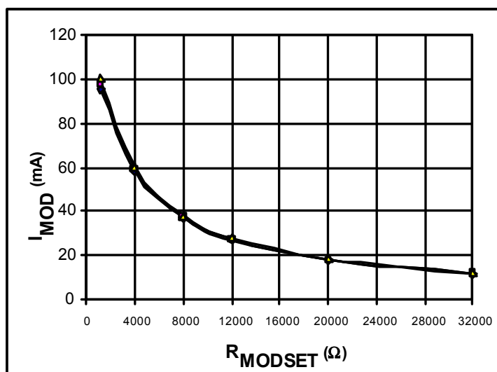
Figure 3-2. Modulation Current for Given R_{MODSET} Resistor
