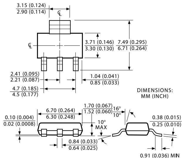
SOT-223 (S)
