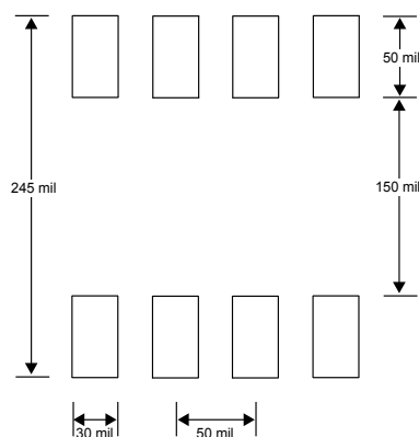
Minimum recommended board pad size, SO-8.
