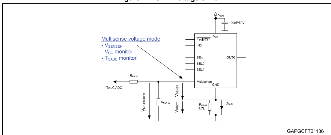
Figure 41: GND voltage shift
