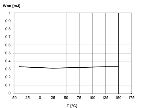
Figure 29: W_{on} vs. T_{case}
