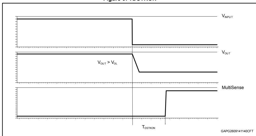
Figure 9: TDSTKON
