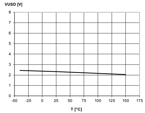
Figure 24: Undervoltage shutdown
