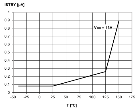
Figure 16: Standby current
