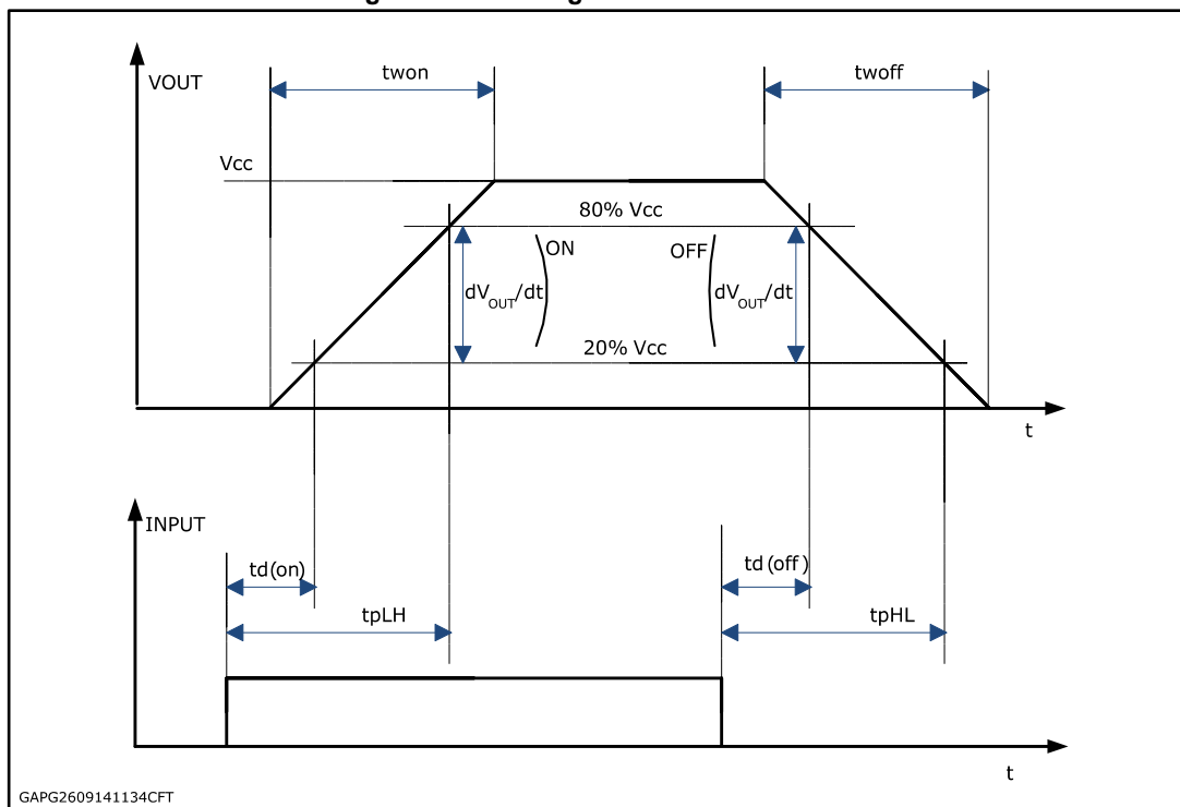
Figure 6: Switching time and Pulse skew
