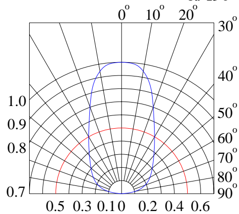
Radiation Diagram
