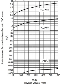
Figure 4-Typical Reverse Characteristics
