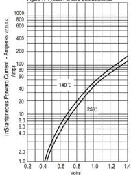
Figure 1-Typical Forward Characteristics
