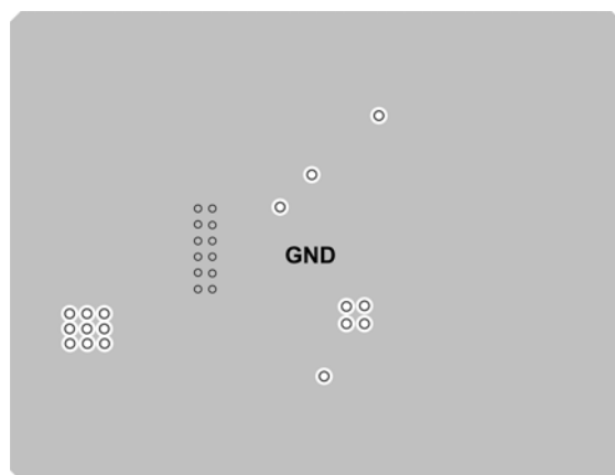
Inner layer-2
