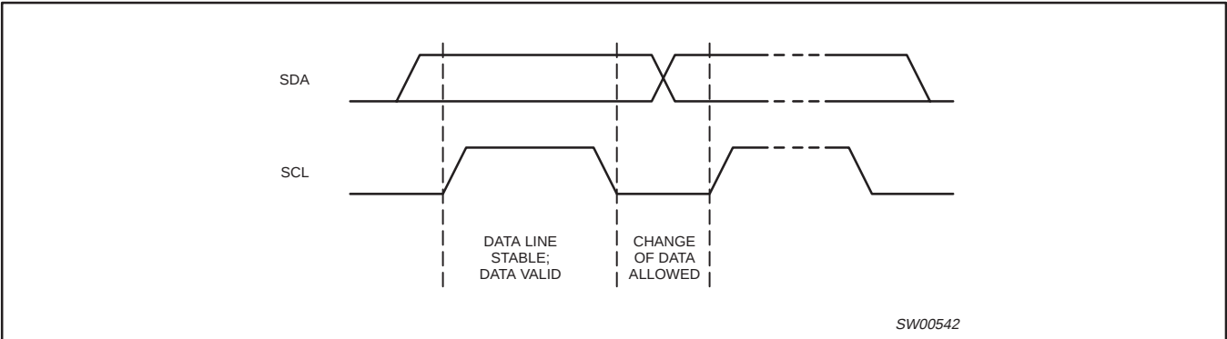
Figure 14. Bit transfer
