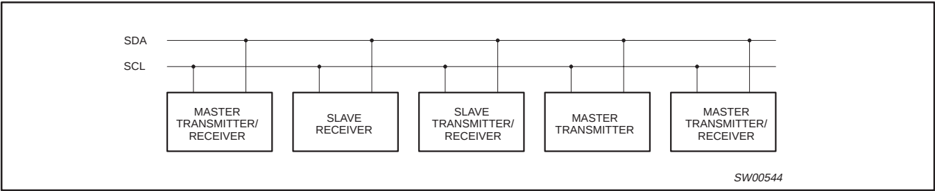
Figure 16. System configuration
