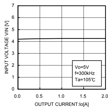
Fig.18 The lowest voltage of possible operation (All series)
