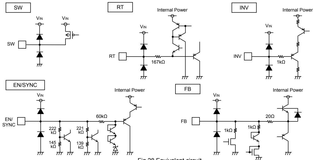
Fig.28 Equivalent circuit
