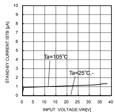
Fig.6 Standby Current (All series)
