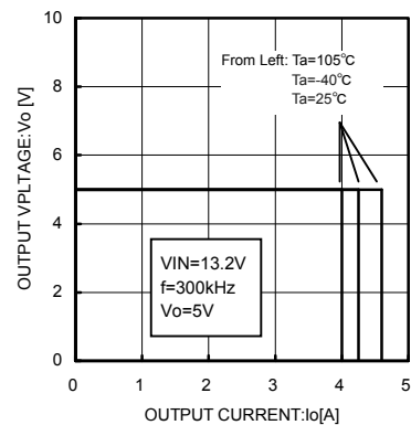
Fig.15 Over-current Protection Operation Current (All series)
