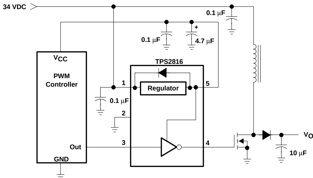
The TPS2816 and TPS2818 drivers include active pullup circuits on the inputs to eliminate the need for external pullup resistors when using controllers with open-collector outputs (such as the TL5001). The TPS2817 and TPS2819 drivers have standard CMOS inputs providing a total device operating current of less than 50 \mu\text{A} . All devices switch at standard CMOS logic levels of approximately 2/3 V_{\text{CC}} with positive-going input levels, and approximately 1/3 V_{\text{CC}} with negative-going input levels. Being CMOS drivers, these devices will draw relatively large amounts of current (Approximately 5 mA) when the inputs are in the range of one-half of the supply voltage. In normal operation, the driver input is in this range for a very short time. Care should be taken to avoid use of very low slew-rate inputs, used under normal operating conditions. Although not destructive to the device, slew rates slower than 0.1 V/ \mu\text{s} are not recommended.
