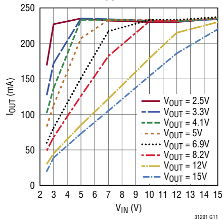
Maximum Output Current vs V_{IN} and V_{OUT}
