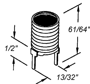
For printed circuit board applications. 05-35 requires two 0.070" holes spaced 0.375" apart.
