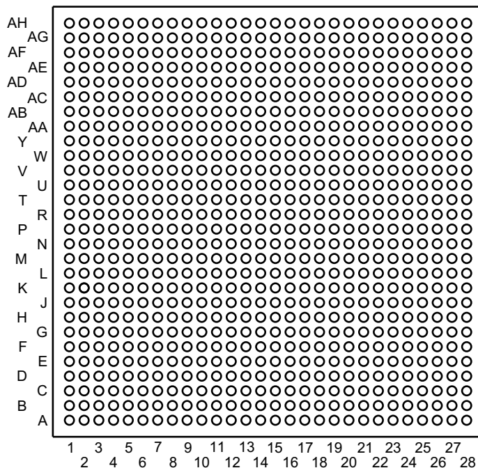
Figure 6-1. ACD FCBGA-N784 Package (Bottom View)
