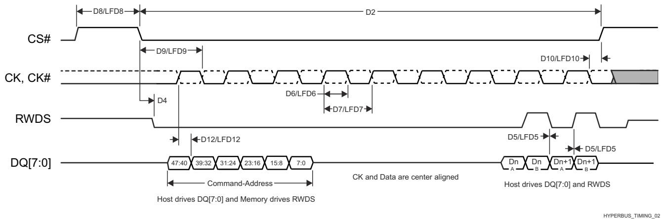
Figure 7-64. HyperBus Timing Diagrams - Receiver Mode
