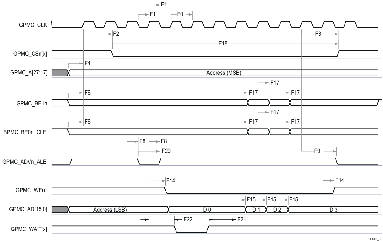
Figure 7-51. GPMC and Multiplexed NOR Flash—Synchronous Burst Read
