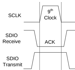
Figure 26: Valid Acknowledge
