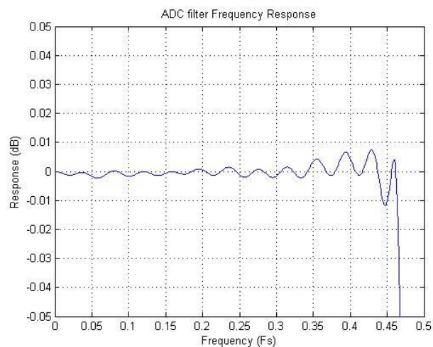
Figure 55: ADC Filter Ripple
