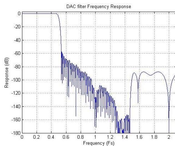
Figure 53: ADC Filter Frequency Response
