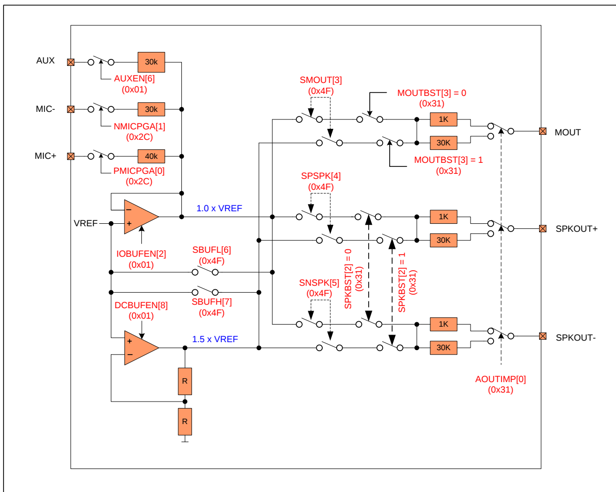
Figure 20: Tie-off Options for the Speaker and MONO output Pins
