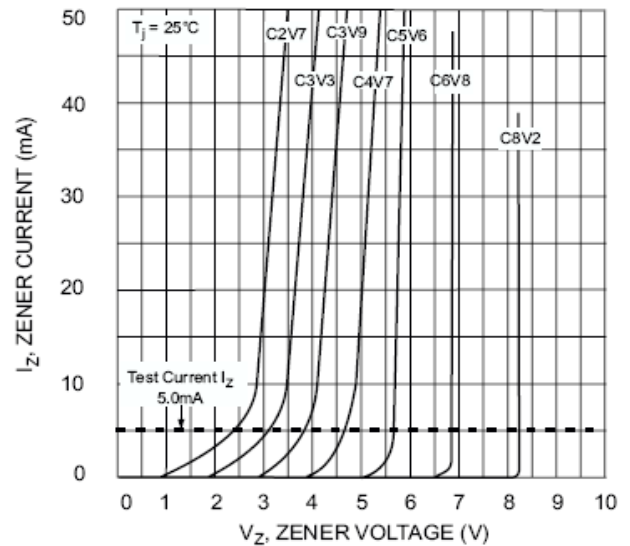
Fig. 2 Zener Breakdown Characteristics
