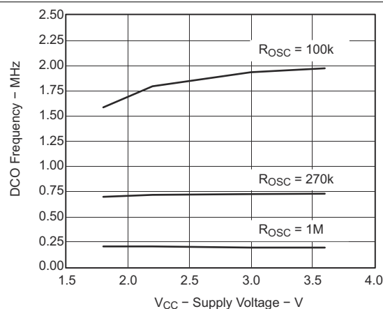
图 8-22. DCO Frequency vs Supply Voltage ( T_A = 25^\circ\text{C} )
