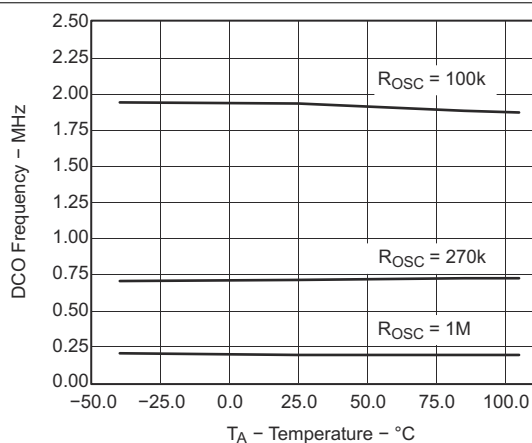
图 8-21. DCO Frequency vs Temperature ( V_{CC} = 3\text{ V} )
