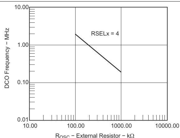
图 8-20. DCO Frequency vs R_{OSC} ( V_{CC} = 3\text{ V} , T_A = 25^\circ\text{C} )
