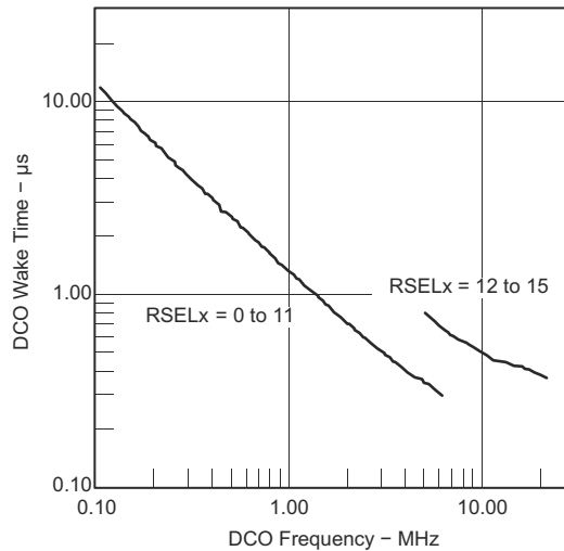
图 8-18. DCO Wake-up Time From LPM3 vs DCO Frequency
