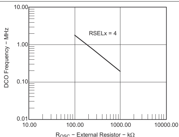
图 8-19. DCO Frequency vs R_{OSC} ( V_{CC} = 2.2\text{ V} , T_A = 25^\circ\text{C} )
