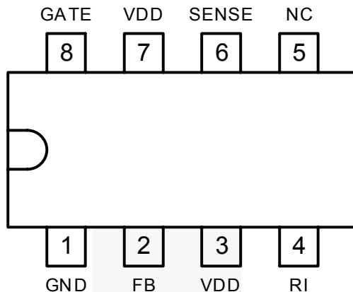
Figure 3. Pin Configuration(Top View)
