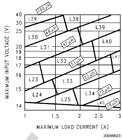
FIGURE 5. LM2676-12EP
