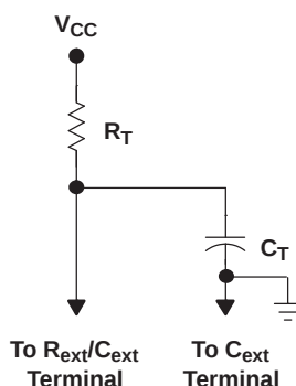
Figure 2. Timing-Component Connections
