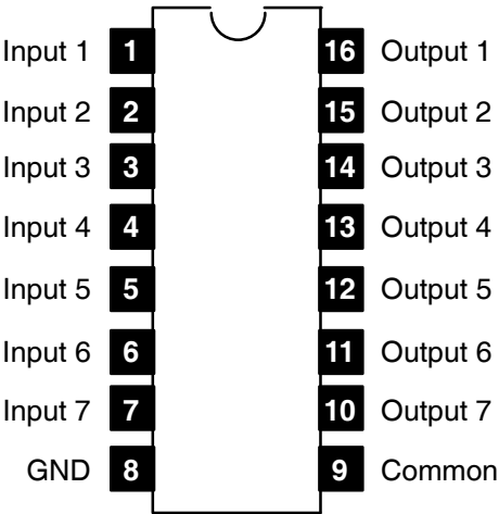
Pin Connection Diagram
