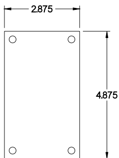
INNER PANEL
